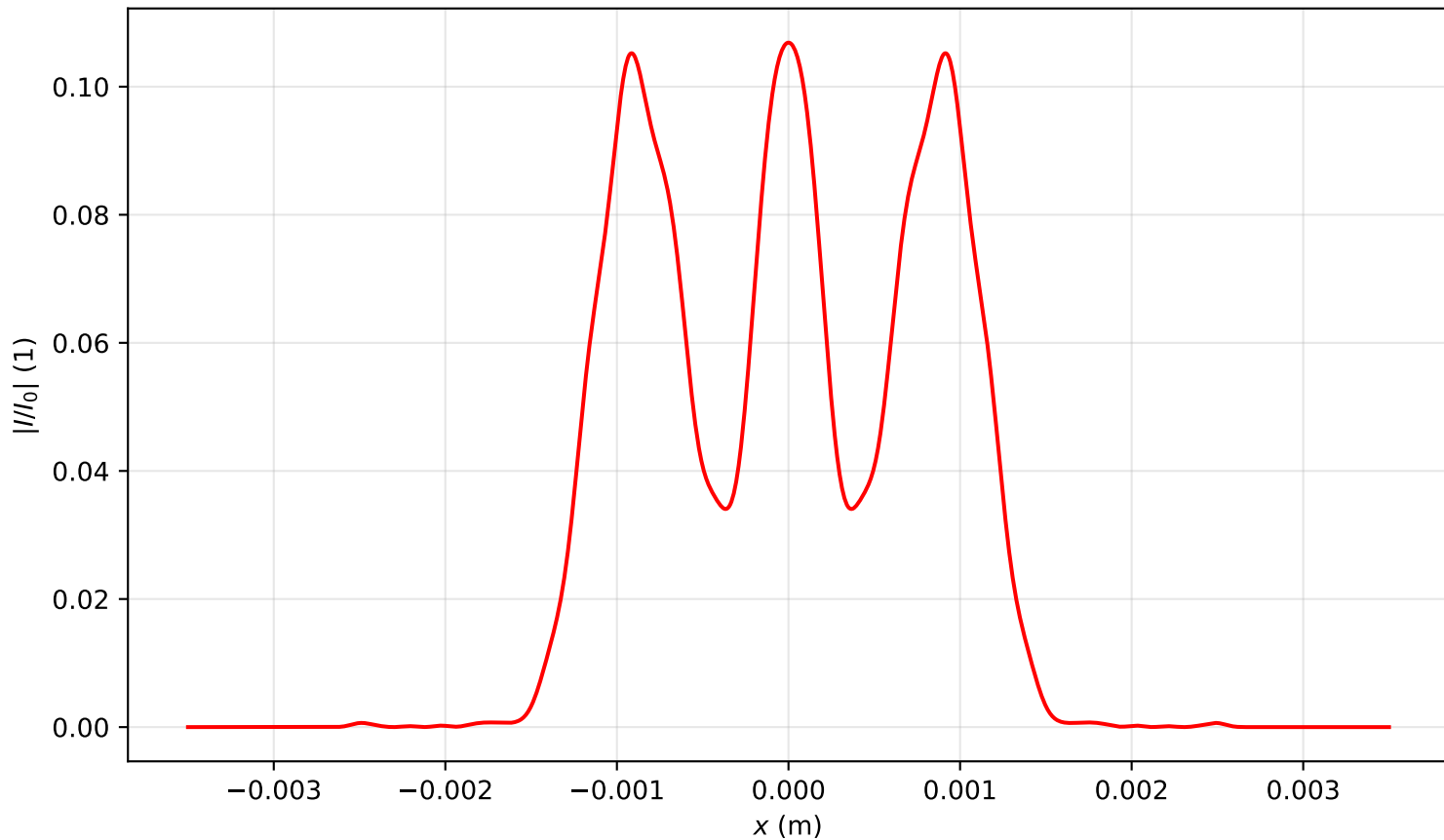
Intensity profile I(x, y = 0, z = 2.388)/I_0 , P_{in}=7.5P_{cr} , artificial time
